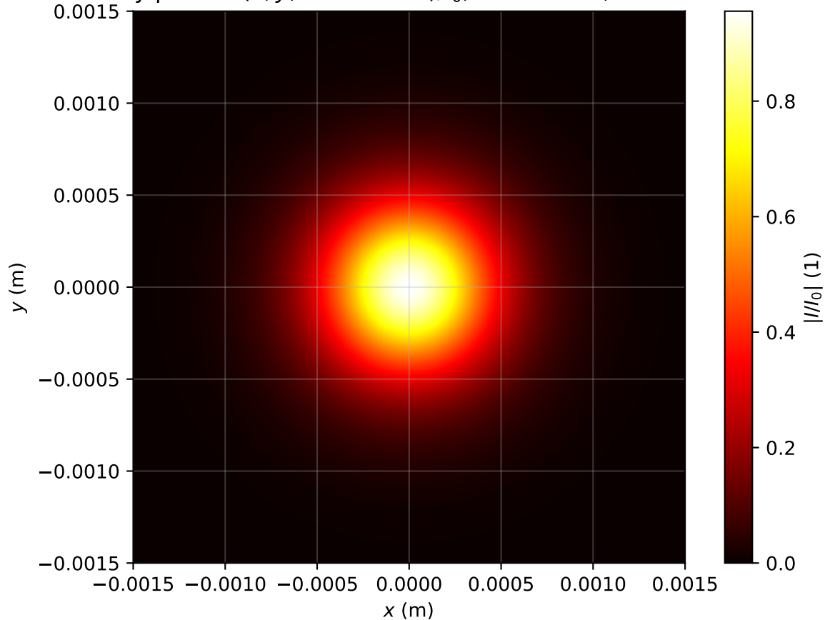
Intensity profile I(x, y, z = 1.513m)/I_0 , P_{in}=0.5P_{cr} , artificial time
